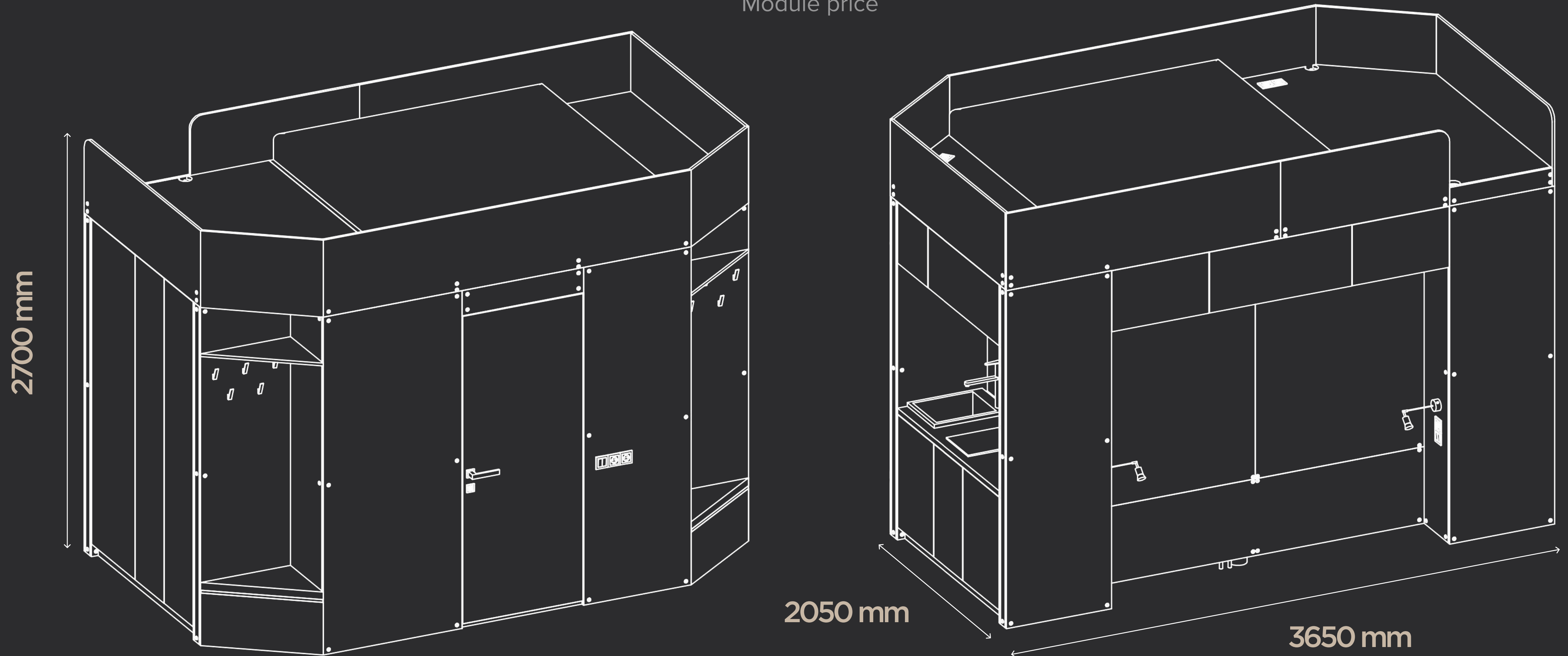
Isometric image of the main unit of the indoor module
